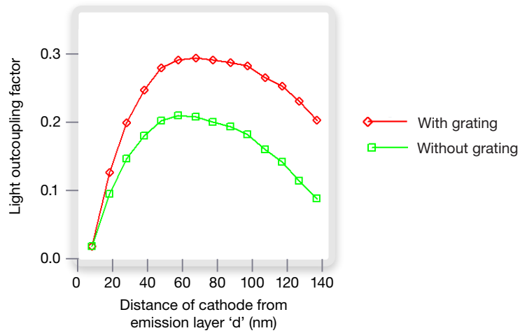
Figure 9: Light out-coupling into air using mixed-level simulation with (red line) and without (green line) the moth's eye grating.
