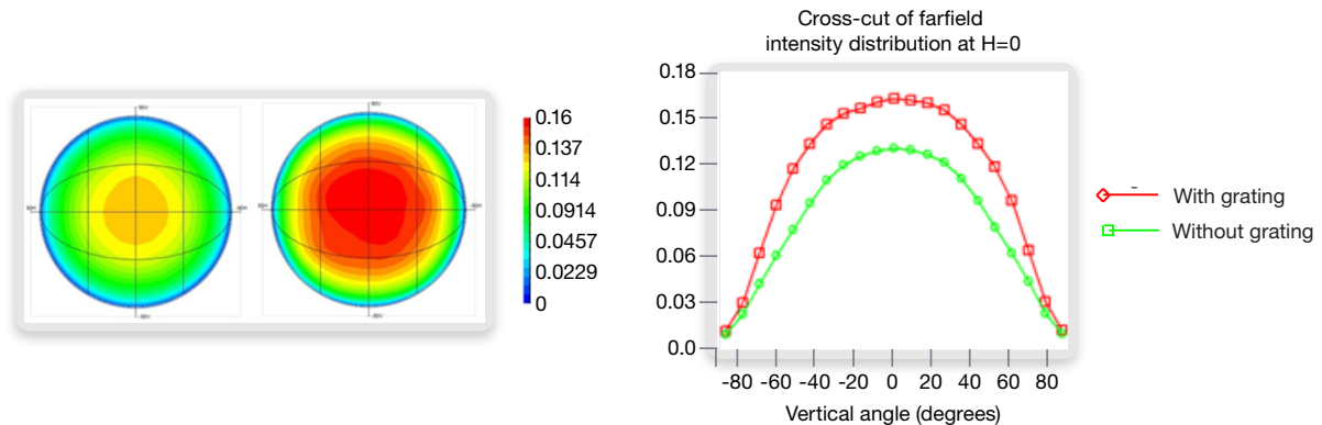
Figure 10: Calculated angular far-field intensity for (a) the Flat interface structure versus (b) the moth's eye grating. (c) Cross-cut at horizontal angle (H=0), showing enhanced out-coupling and improved angular uniformity.
